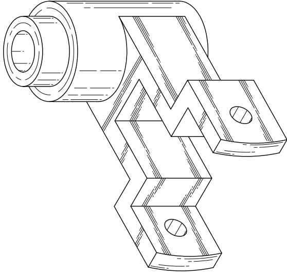
PERSPECTIVE VIEW
