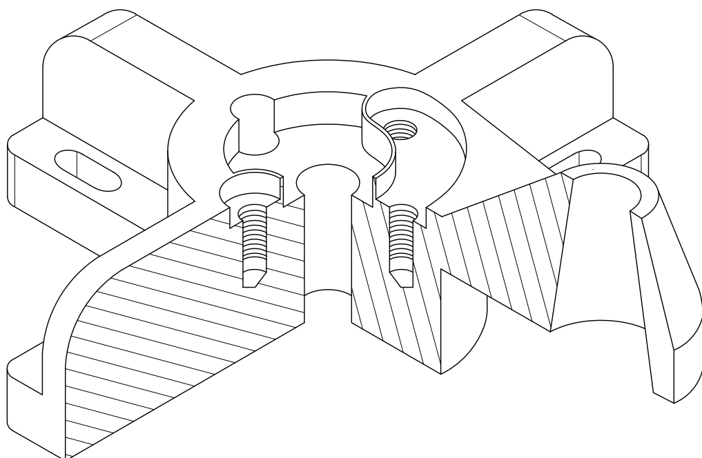
Sectional View FIG. 30
